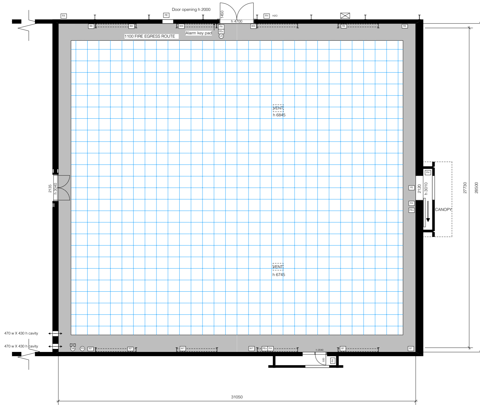
PLAN AT 1:100
