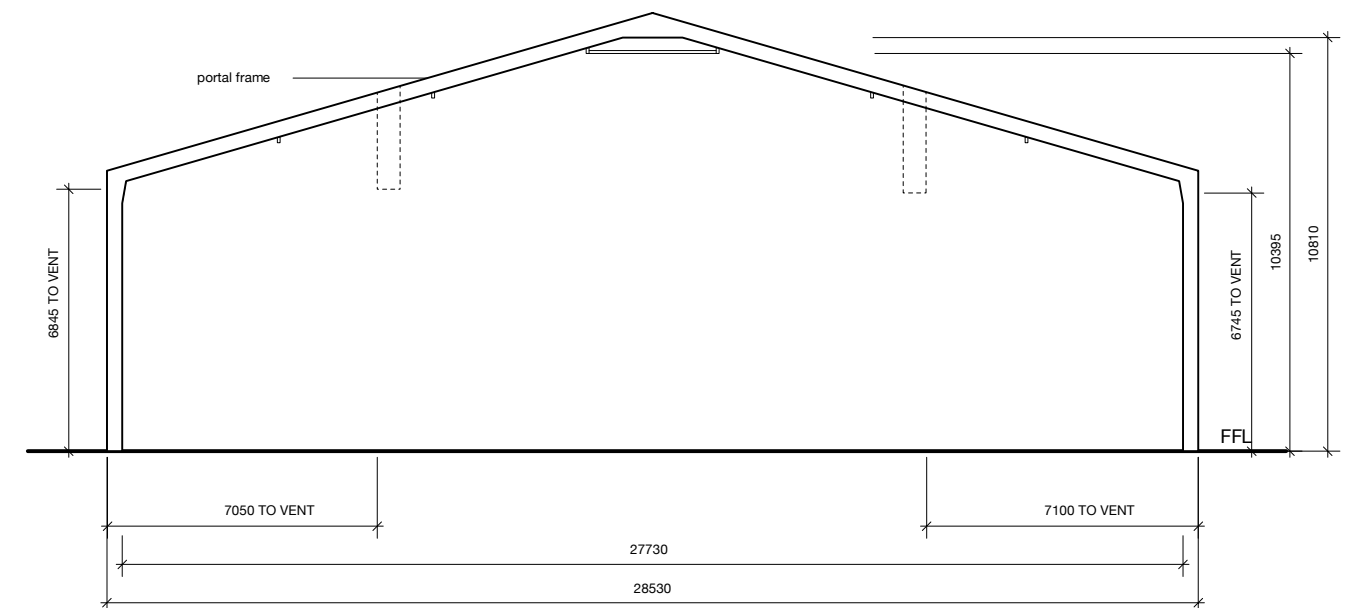
SECTION AT 1:100
